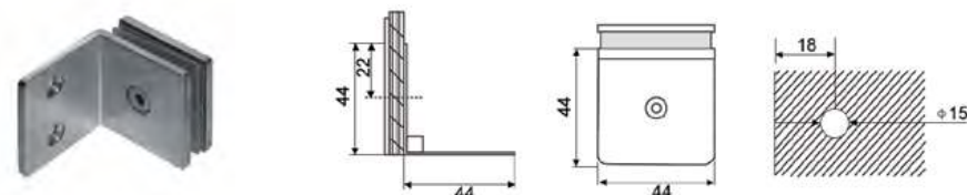
Spojnica kutna zid- staklo 90° inox SAT / inox POL debljina stakla 8/10 mm
