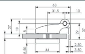
Spojnica ALU/staklo nikal mat (inox) debljina stakla 8/10 mm
