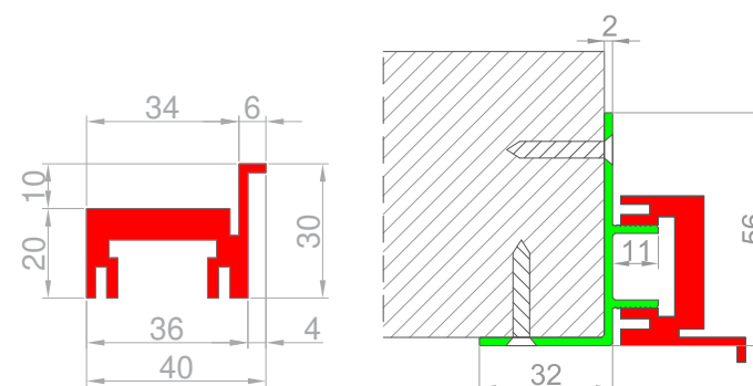
Alu dovratnik "INVISIBLE"
