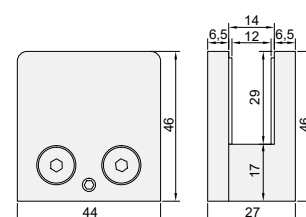
Spojnica zid - staklo inox POL / SAT debljina stakla 10 mm
