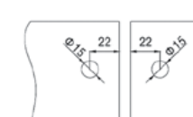
Spojnica ravna staklo - staklo inox POL / SAT debljina stakla 8/10/12 mm
