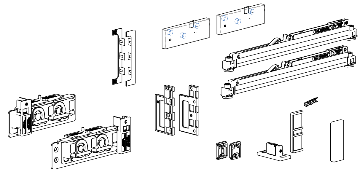
V Diva Fluid set staklo set
