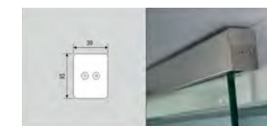
Stoper
