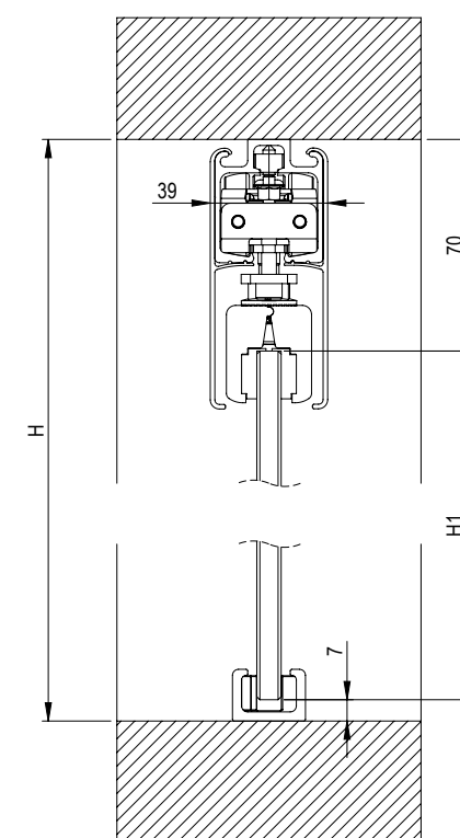
Porta Glass SLX set stakleno krilo
